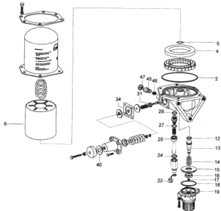
AIR DRYER WITH TYRE INFLATOR
