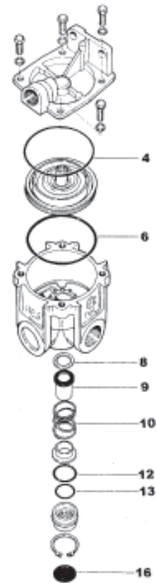
RELAY VALVE (NEW - RG2)
