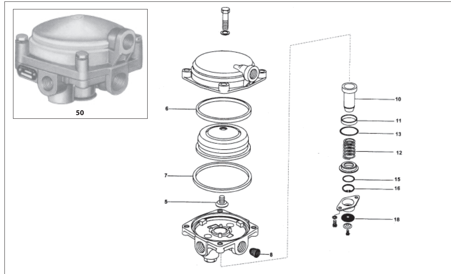
RELAY VALVE (OLD - R6)
