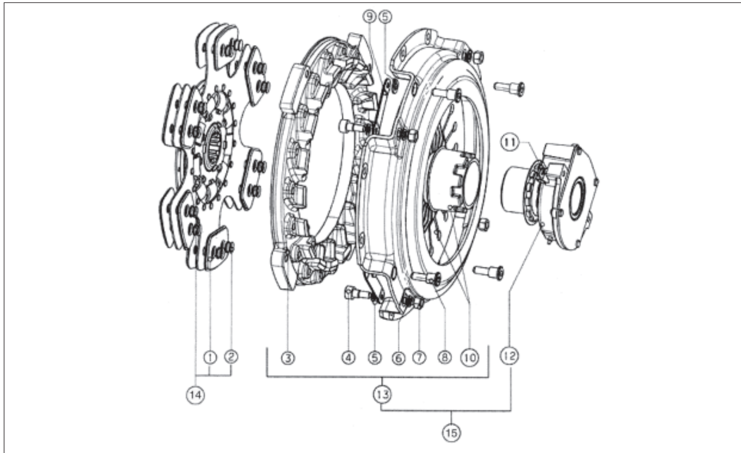
CLUTCH (352 DIA.) DIAPHRAGM TYPE
