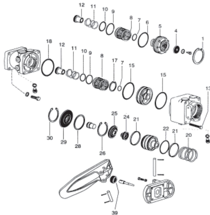
DUAL TREADLE VALVE WITH INTEGRAL FILTER (COWL)
